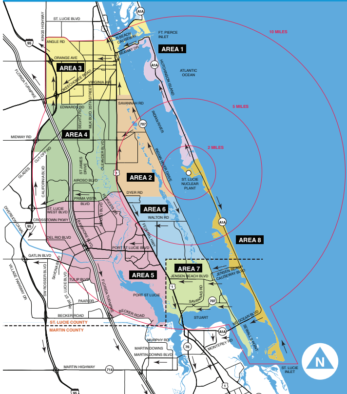
Power Plant 10-Mile Radius and Evacuation Areas
