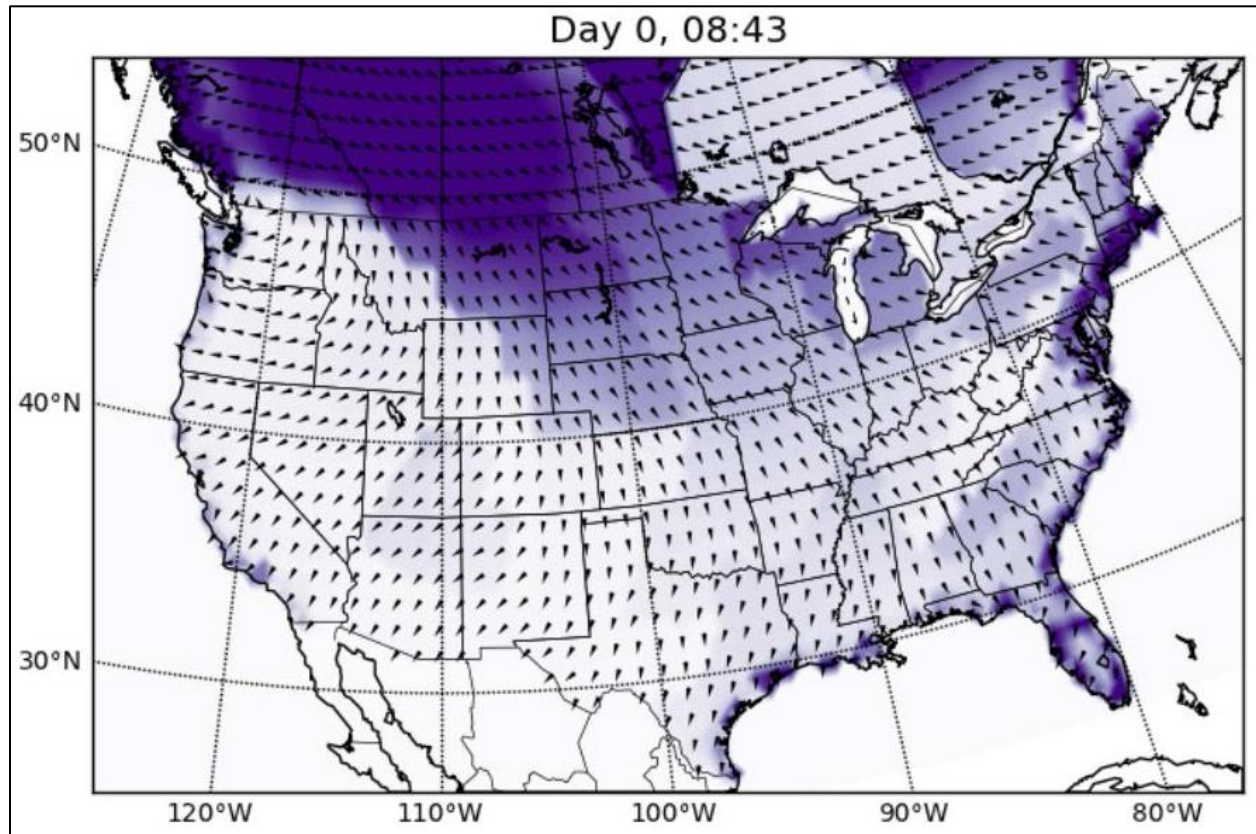
Figure 102: Carrington Level Storm Electric Field Amplitudes Model 292
