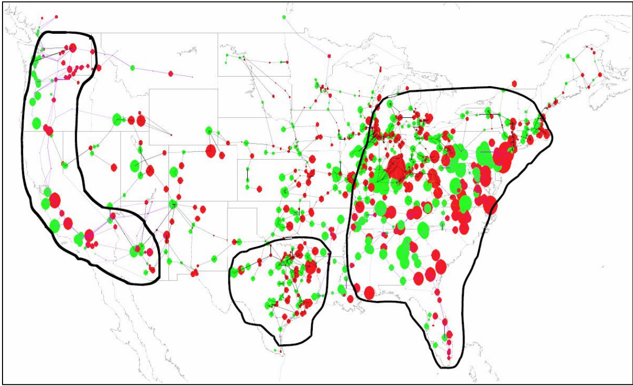
Figure 100: United States Regions Susceptible to Electric System Collapse, 100-year Geomagnetic Storm 45 degree Latitude Scenario, 290
