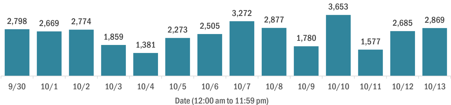
7-day average number of cases
