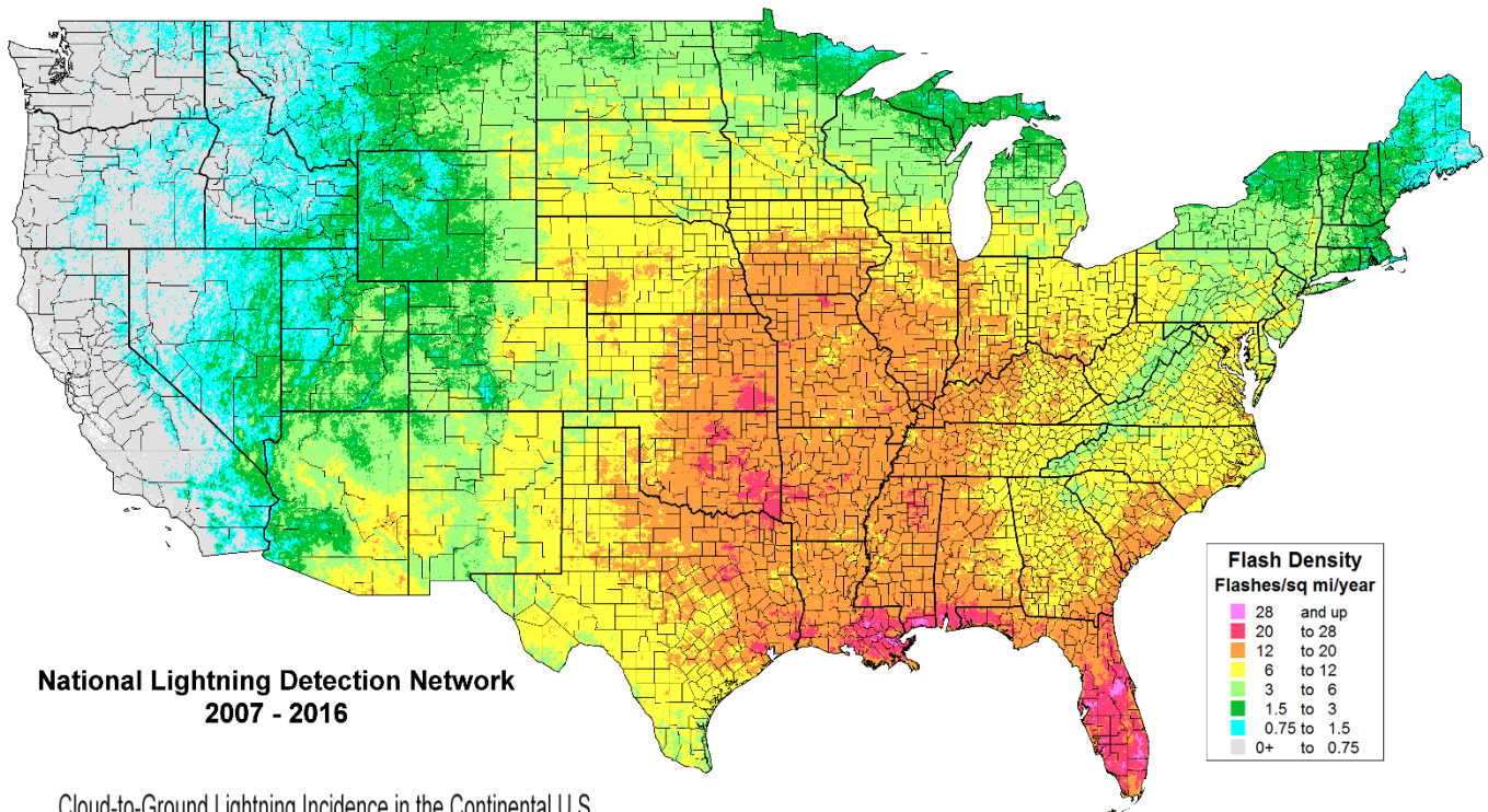
Cloud-to-Ground Lightning Incidence in the Continental U.S.
